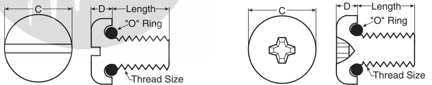
(S) Slotted Pan Head
